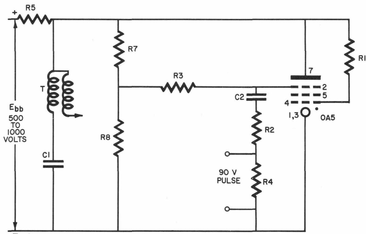
FIGURE 1—FIXED TRIGGER GRID BIAS
