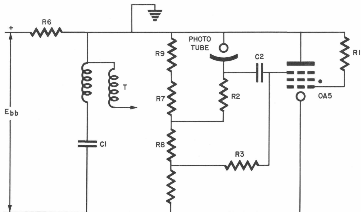
FIGURE 3—PHOTOTUBE TRIPPING CIRCUIT
