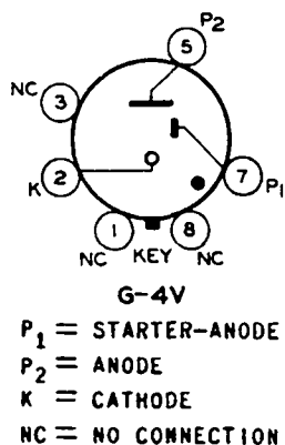
BOTTOM VIEW OF SOCKET CONNECTIONS
