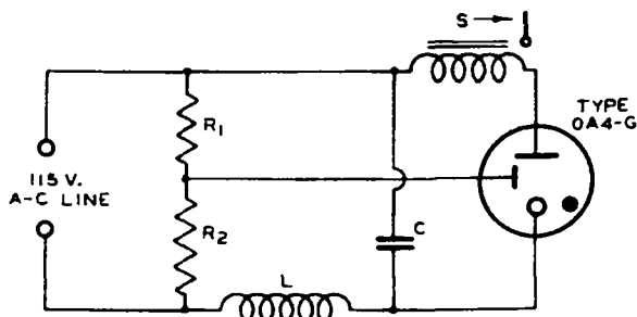
SCHEMATIC RELAY CIRCUIT USING TYPE 0A4-G A-C OPERATION
