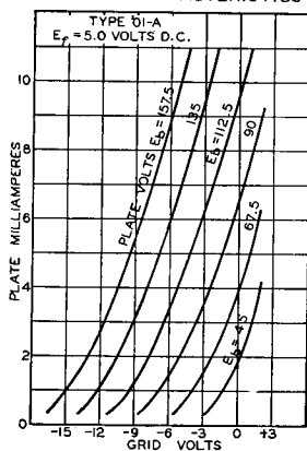
AVERAGE PLATE CHARACTERISTICS
