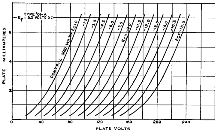
AVERAGE CHARACTERISTICS
