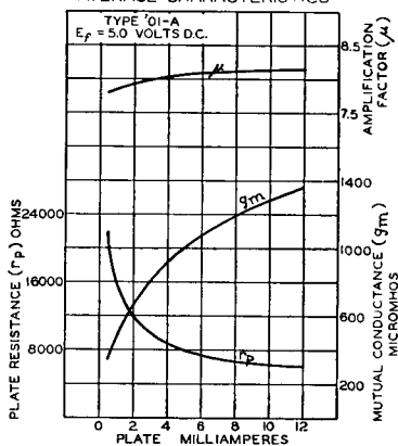
AVERAGE PLATE CHARACTERISTICS
